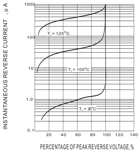
Fig. 3-TYPICAL REVERSE CHARACTERISTIC
