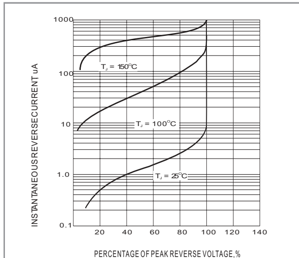
Fig.4-TYPICAL REVERSE CHARACTERISTIC
