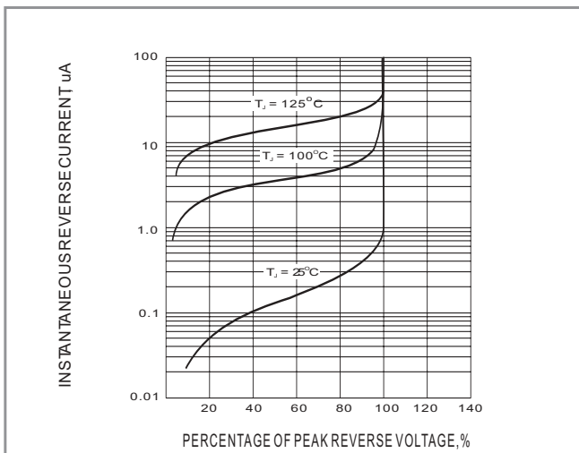
Fig.3-TYPICAL REVERSE CHARACTERISTIC
